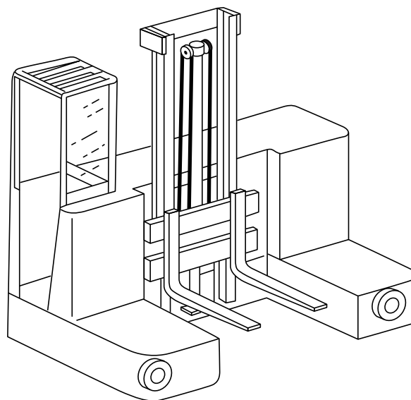
Fig. 21 Single Side Loader Rider Truck
