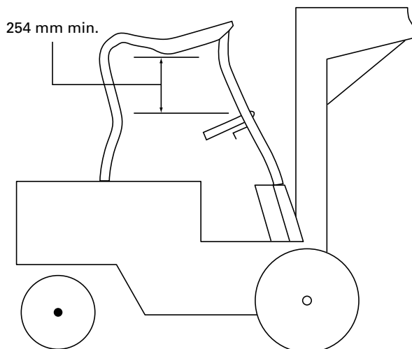
Fig. 6 Overhead Guard Impact Deformation Limit (Sit-Down)
