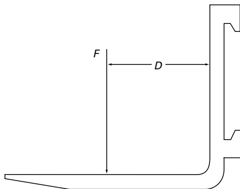
Fig. 3 Typical Fork
