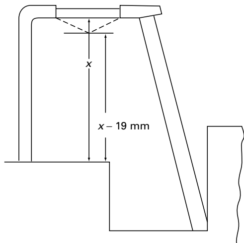
Fig. 4 Overhead Guard Cube Drop Test Deformation Limit
