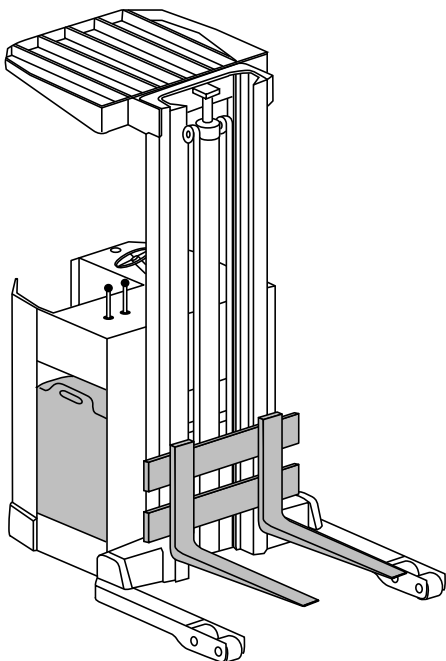
Fig. 18 Narrow Aisle Rider Truck, Straddle Truck
