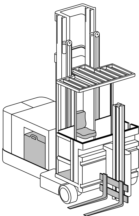
Fig. 19 Operator-Up Counterbalanced Front/Side Loader Truck
