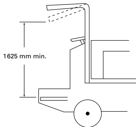
Fig. 7 Overhead Guard Impact Deformation Limit (Stand-Up)
